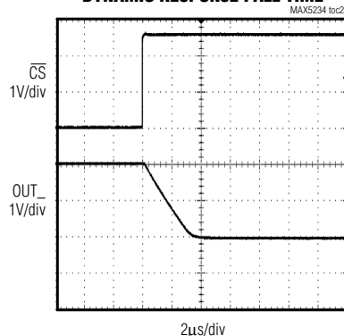
MAX5234 DYNAMIC RESPONSE FALL TIME
