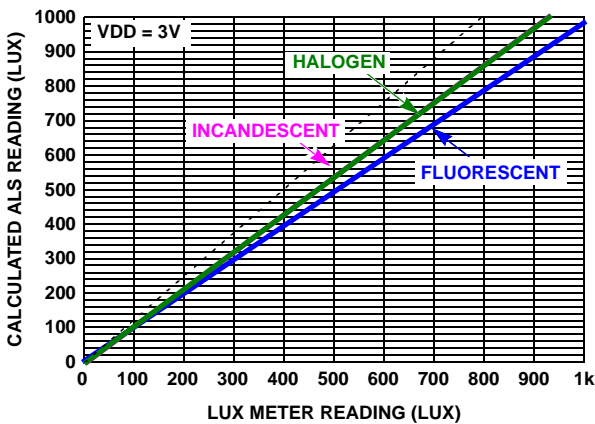
FIGURE 18. LIGHT SENSITIVITY vs LUX LEVEL
