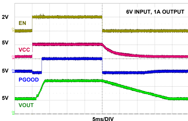
FIGURE 11. ENABLE/DISABLE WAVEFORMS
