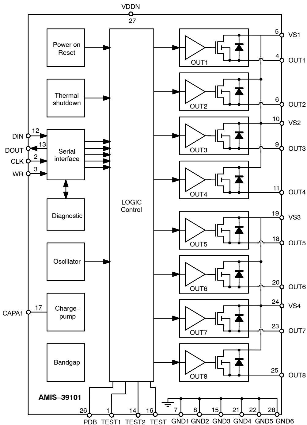
Figure 1. Block Diagram
