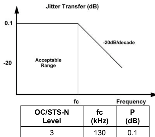
Figure 2. Jitter Transfer
