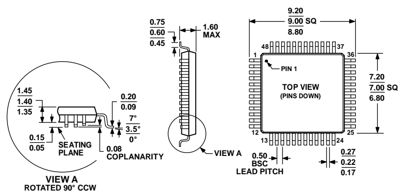
COMPLIANT TO JEDEC STANDARDS MS-026-BBC Figure 60. 48-Lead Low Profile Quad Flat Package [LQFP] (ST-48) Dimensions shown in millimeters
