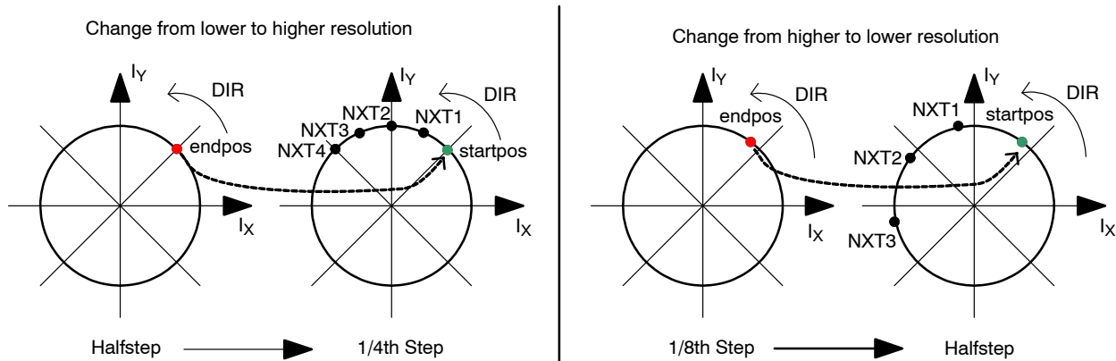
Figure 18. NXT-Step-Mode Synchronization
