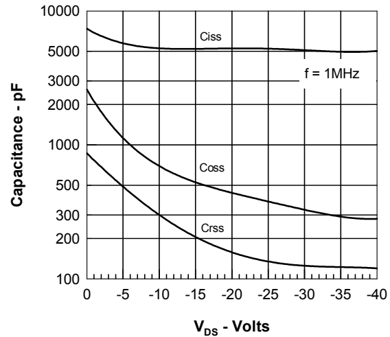
Fig. 8. Capacitance Curves
