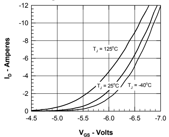
Fig. 6. Admittance Curves
