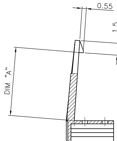
SECTION Z-Z
