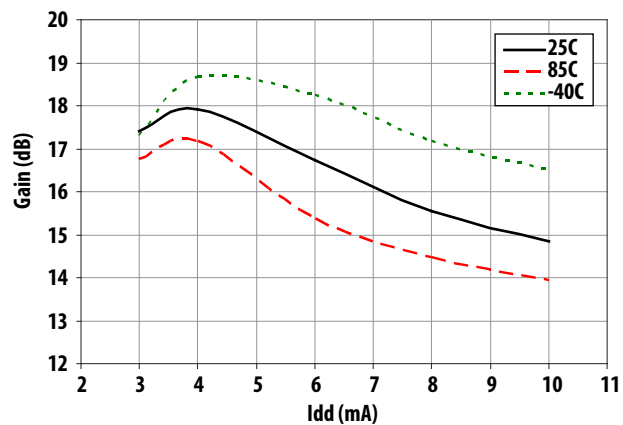
Figure 11. Gain vs. Idd at Vdd = 1.8V
