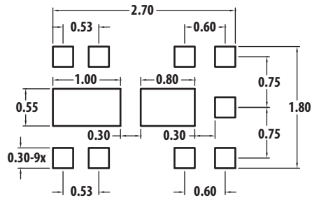
Land Pattern
