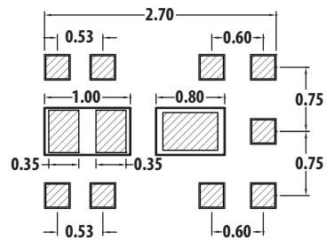
Combination of Land Pattern & Stencil Opening
