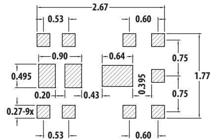
Stencil Opening
