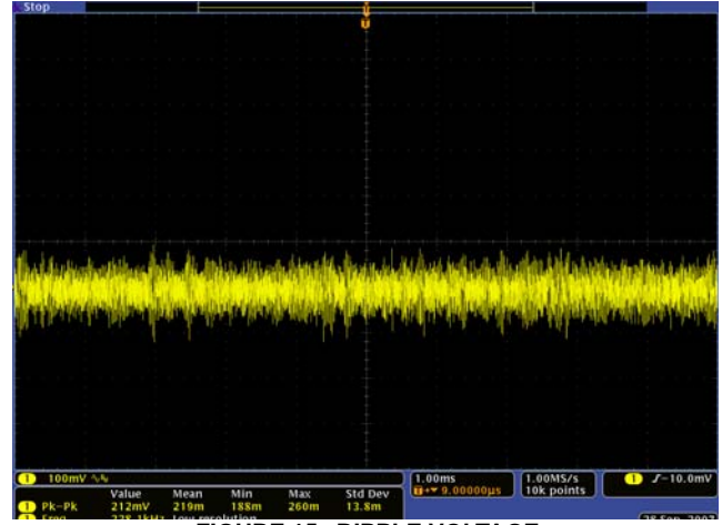
FIGURE 15. RIPPLE VOLTAGE
