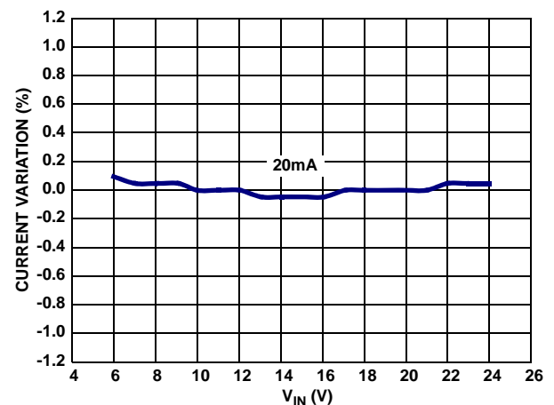
FIGURE 5. CURRENT REGULATION
