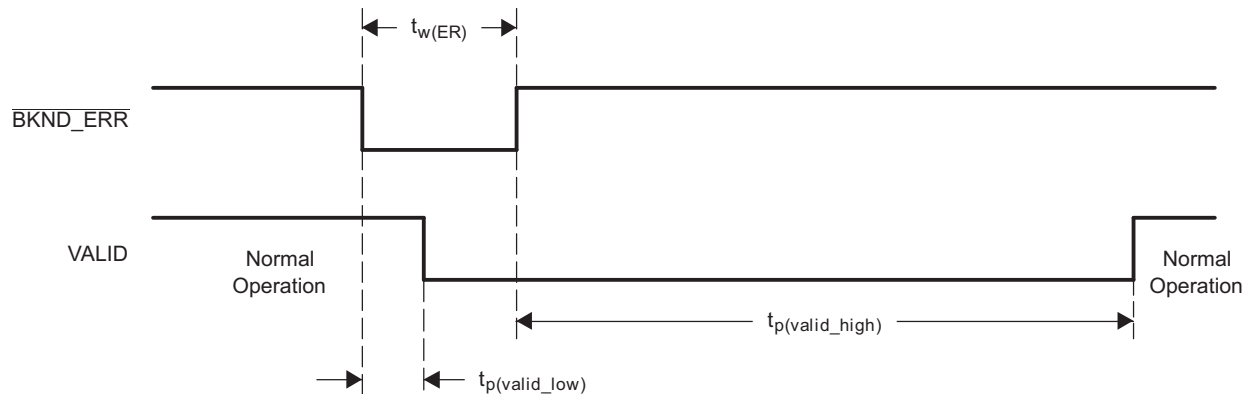
Figure 7-6. Error-Recovery Timing
