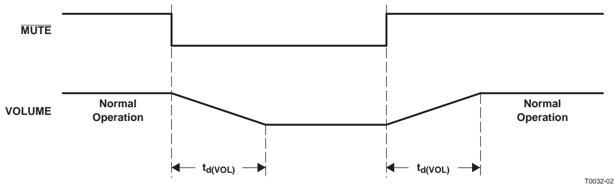
Figure 7-7. Mute Timing
