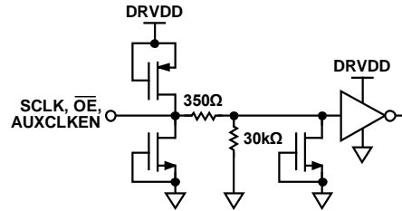
Figure 16. SCLK, OE
