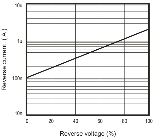
Fig. 2 - Reverse characteristics
