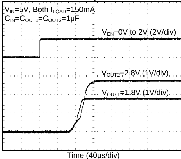
Start-Up Time
