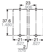
Chassis (Panel) cutout in tandem mounting
