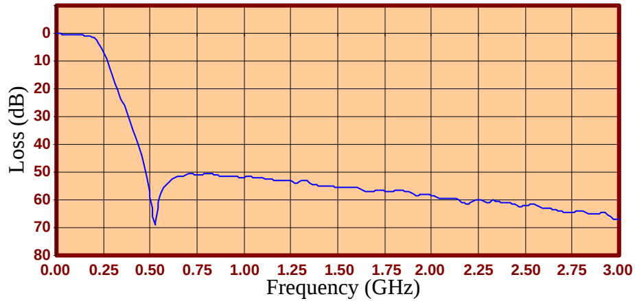
200 MHz Insertion Loss
