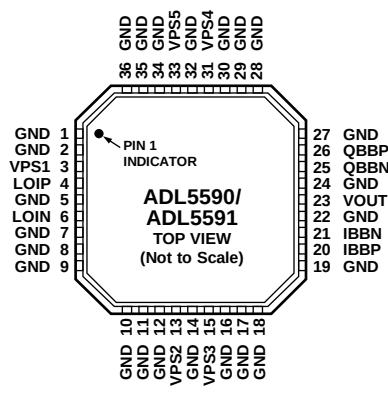
Figure 2. ADL5590/ADL5591 Pin Configuration
