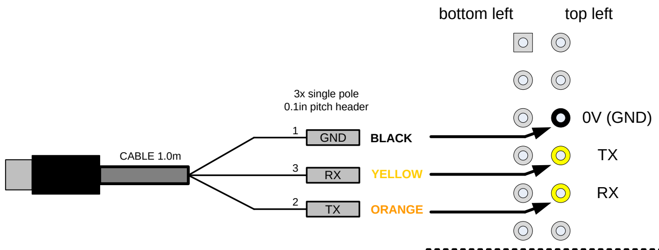
Figure 5-1 – TTL-232R-RPi Debug cable, connection diagram
