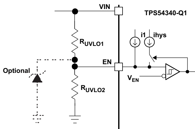
Figure 23. Adjustable Undervoltage Lockout (UVLO)
