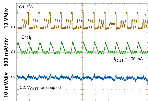
Figure 40. Output Ripple DCM
