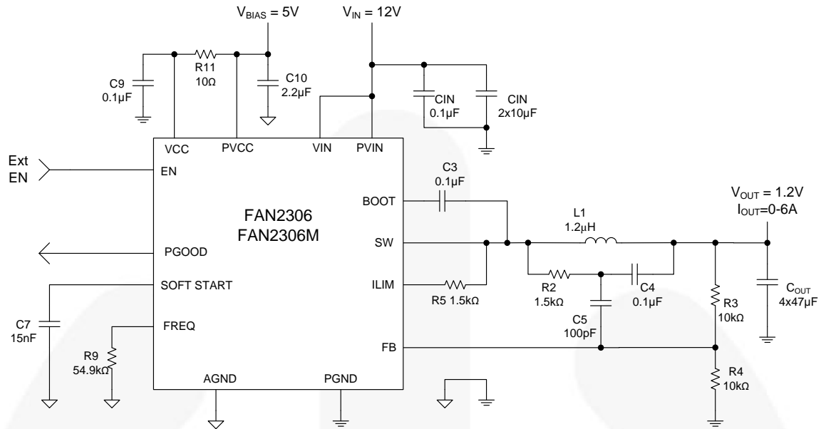
Figure 1. Typical Application
