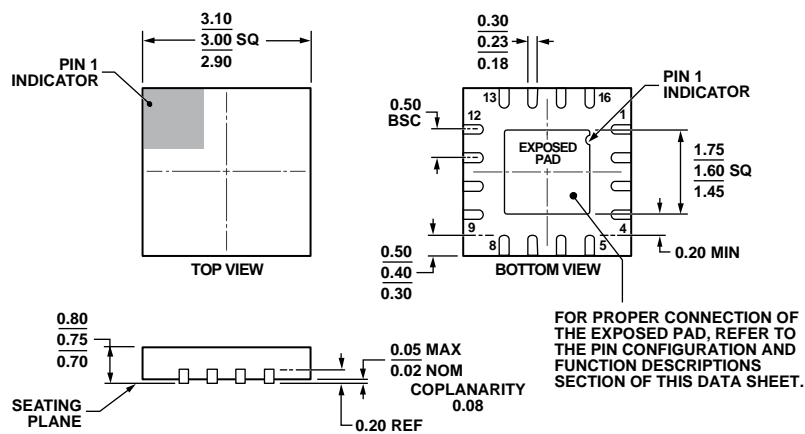
Figure 36. 16-Lead Lead Frame Chip Scale Package [LFCSP_WQ] 3 mm × 3 mm Body, Very Thin Quad (CP-16-22)
