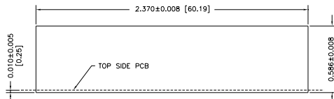
Panel cutout
