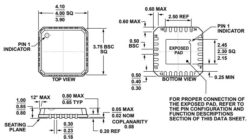
Figure 49. 24-Lead Lead Frame Chip Scale Package [LFCSP_VQ] 4 mm × 4 mm Body, Very Thin Quad (CP-24-2)
