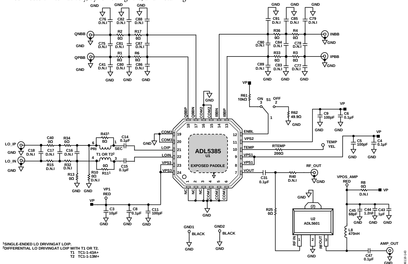
Figure 43. ADL5385-DIFFLO-EBZ Schematic
