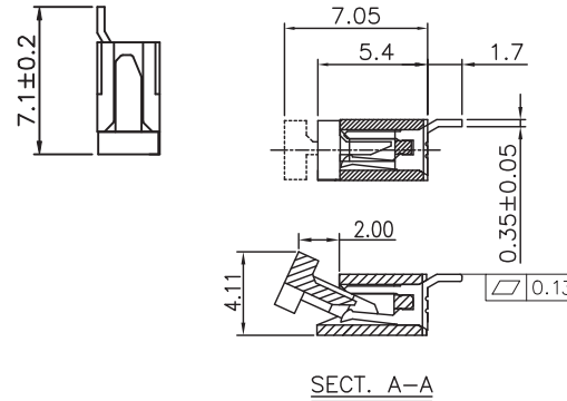
SECT. A-A
