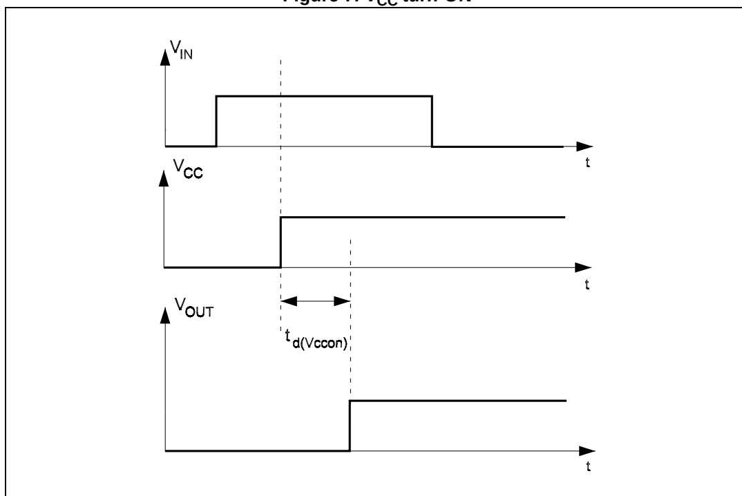
Figure 7. V_{CC} turn-ON
