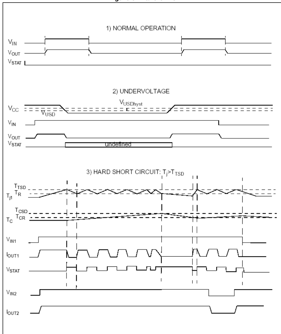
Figure 8. Waveforms
