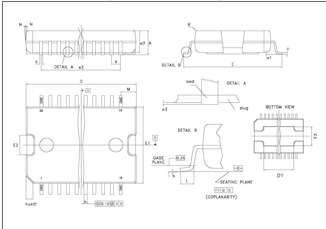
Figure 11. PowerSO-36 drawings
