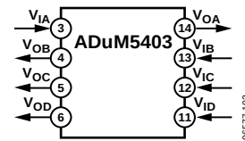
Figure 4. ADuM5403
