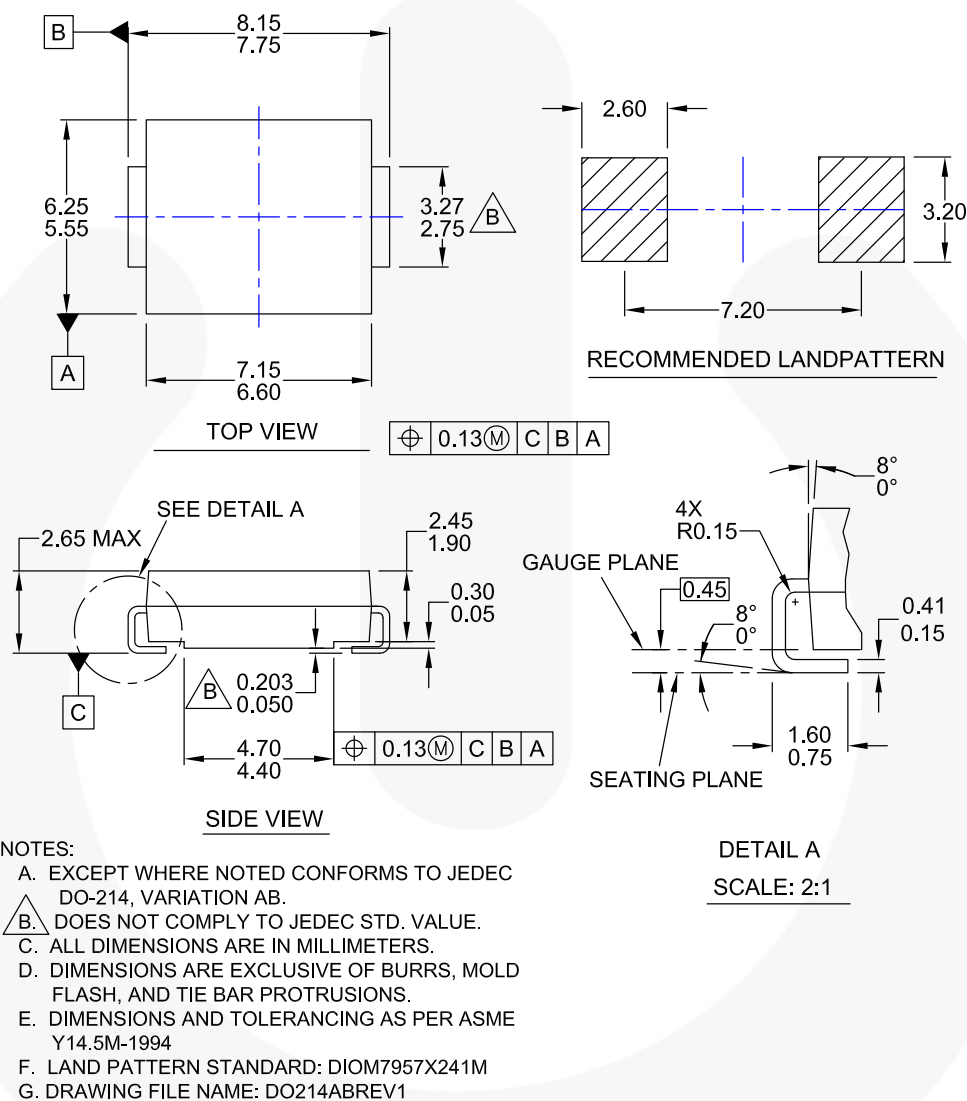
Figure 7. 2-LEAD, SMC, JEDEC DO-214, VARIATION AB (ACTIVE)
