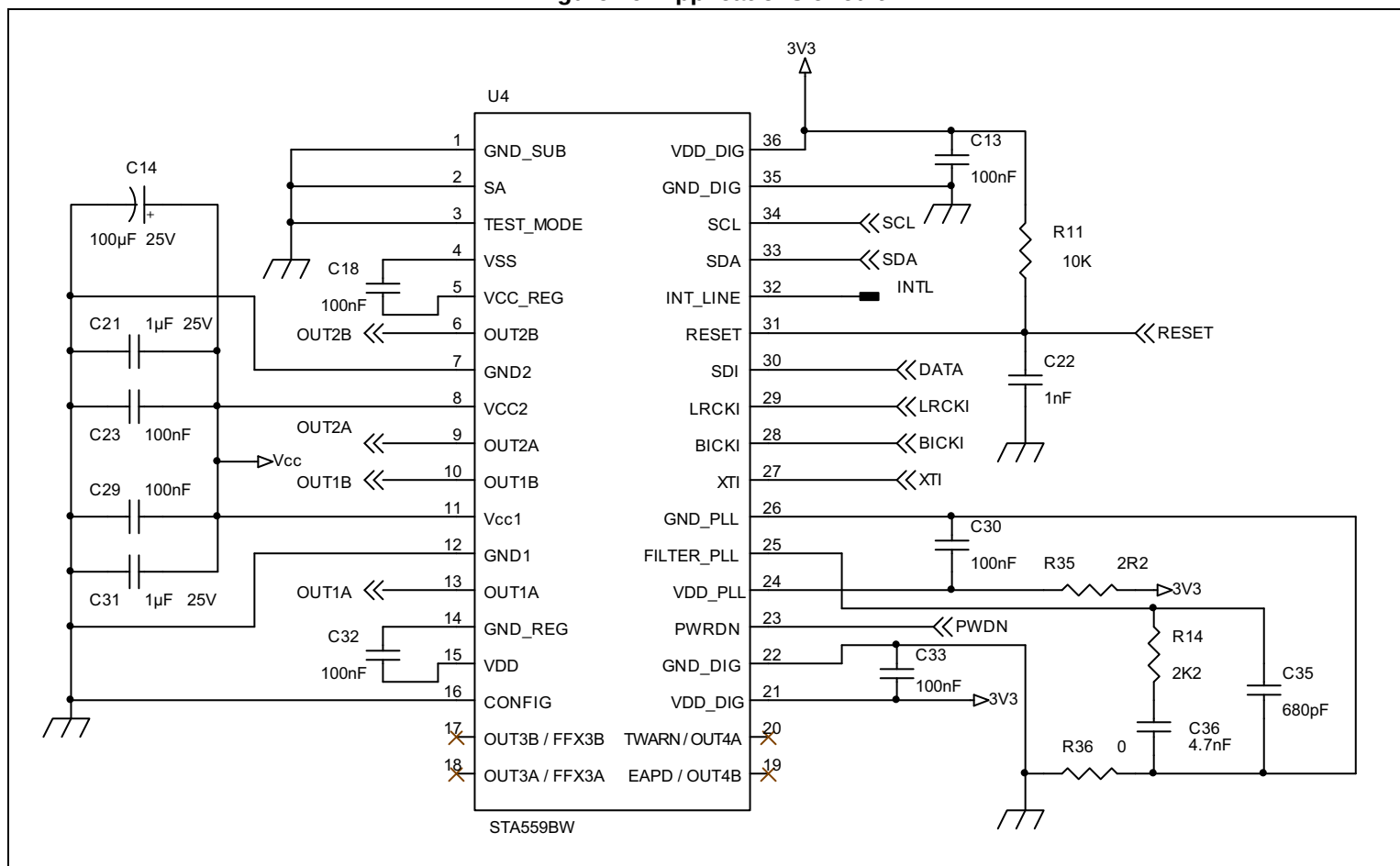
Figure 19. Applications circuit
