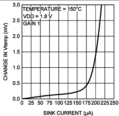
Figure 10. Load Regulation (1)
