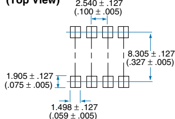
PC Board Pattern (Top View)
