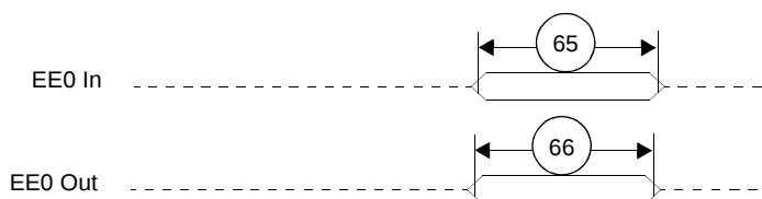
Figure 23. EE Pin Timing
