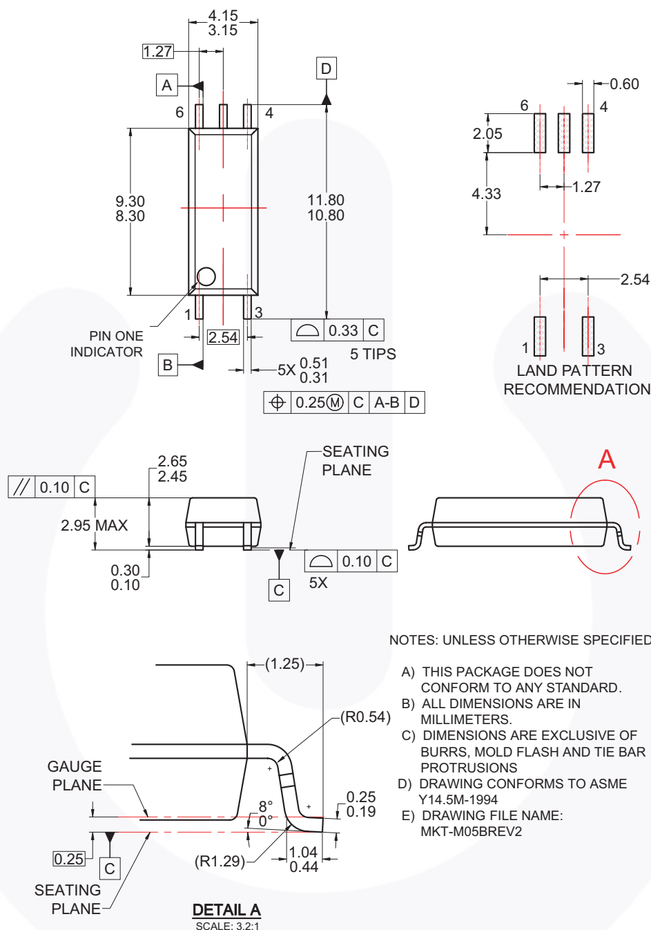
Figure 33. Wide Body SOP 5-Pin
