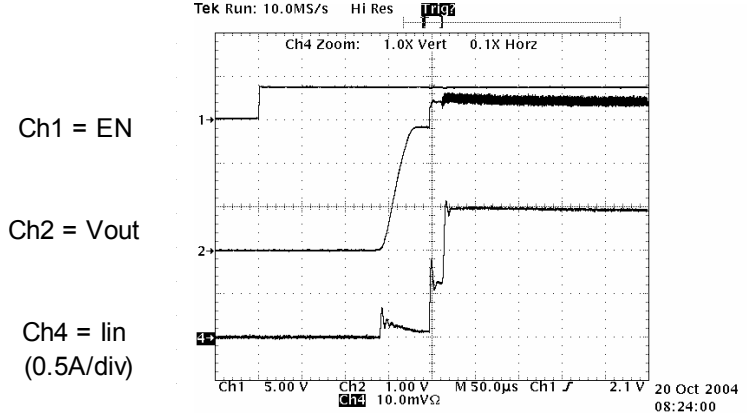
Figure 6. Startup 700mA Flash, Vin=3.6V, Vout=3.3V.
