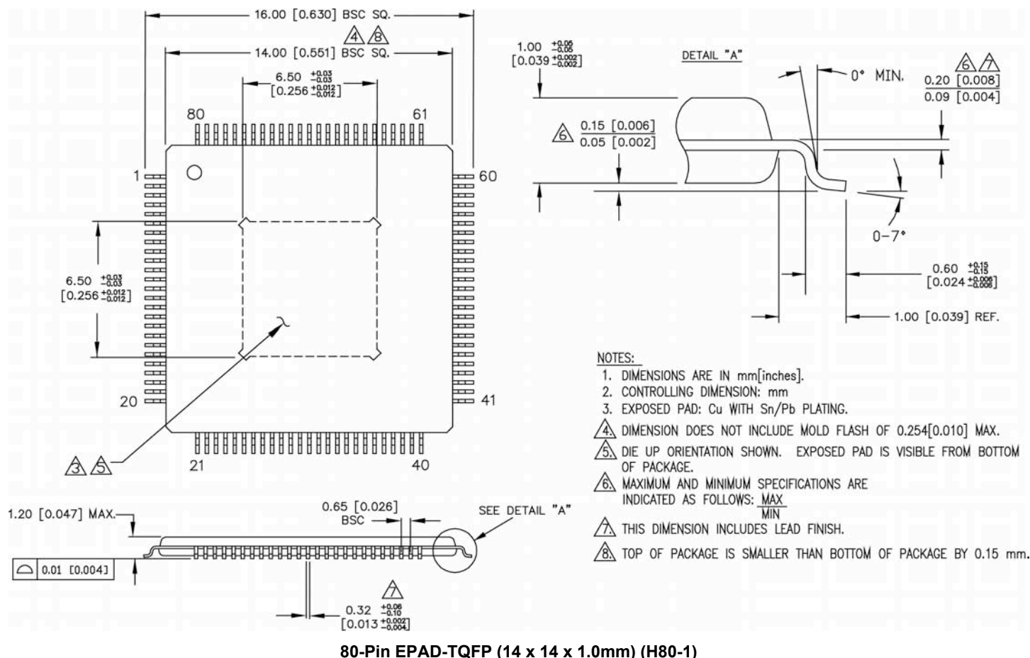
80-Pin EPAD-TQFP (14 x 14 x 1.0mm) (H80-1)
