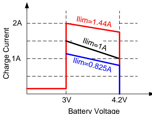
Figure 7— I_{CHG} Variation with Different Input Current Limit
