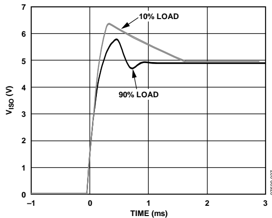
Figure 9. Typical V_{ISO} = 5\text{ V} Output Voltage Start-Up Transient at 10% and 90% Load
