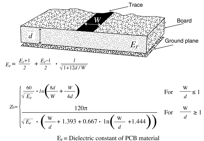
Figure 77: Microstrip Formulas
