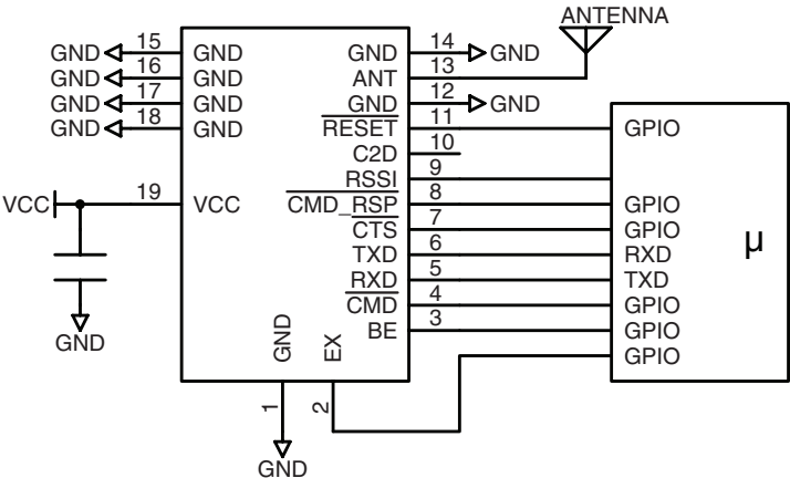
Figure 73: 25 Series Transceiver Basic Application Circuit
