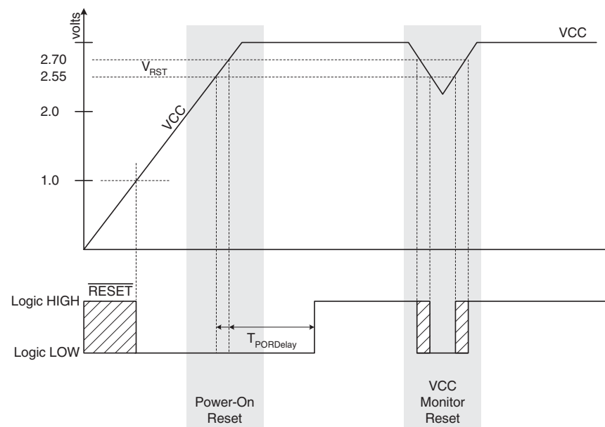
Figure 17: 25 Series Transceiver Reset Timing Diagram
