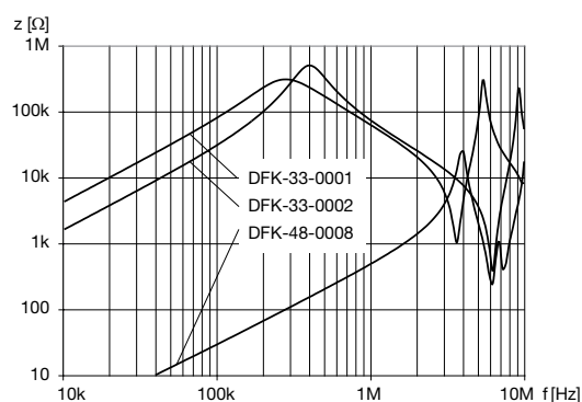
DFK-33-xxxx, DFK-48-xxxxx
