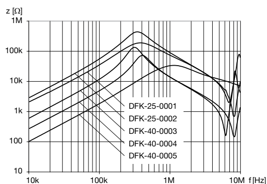
DFK-25-xxxx, DFK-40-xxxxx
