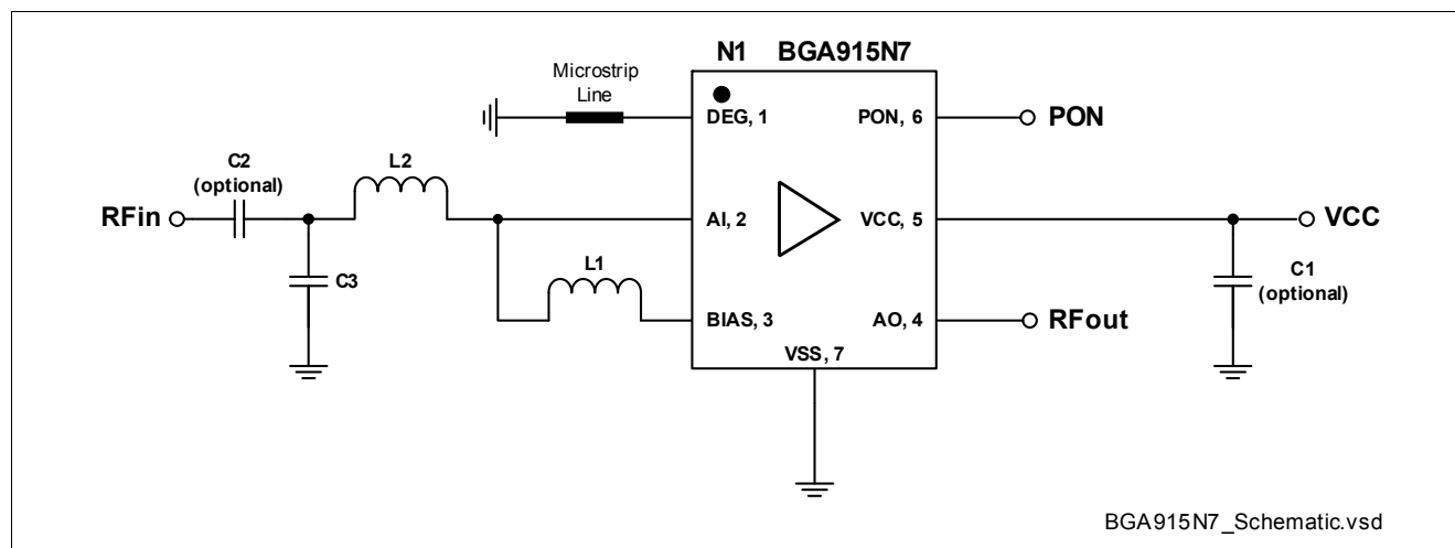
Figure 2 Application Schematic BGA915N7
