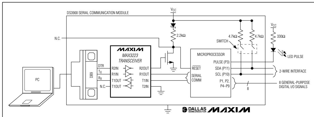
Figure 1. Functional Diagram
