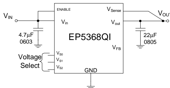
Figure 2: Typical Application Schematic
