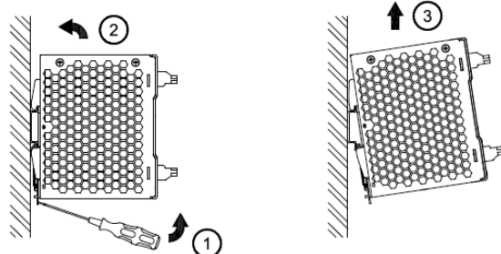
Fig. 2.2 Dismounting
