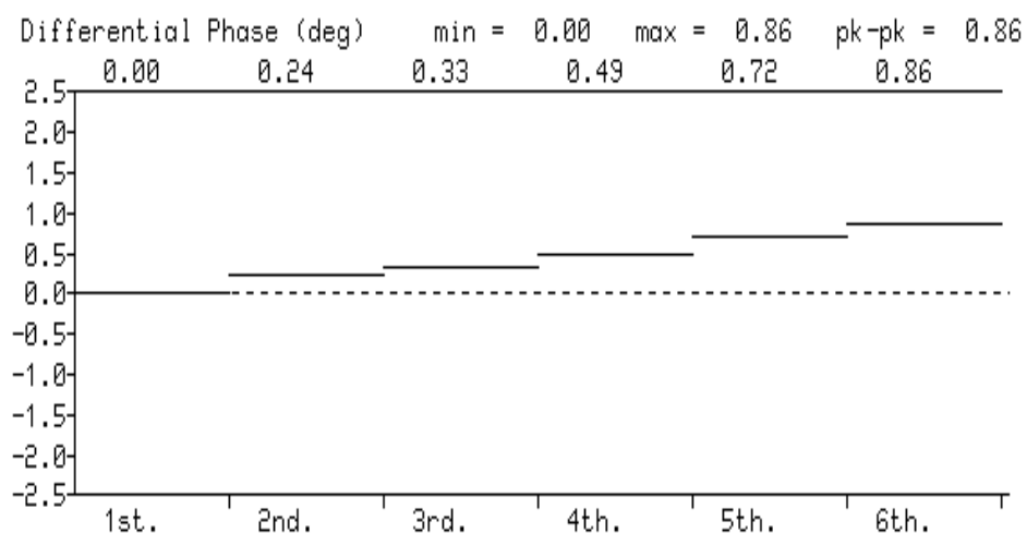
Figure 12. Differential Phase
