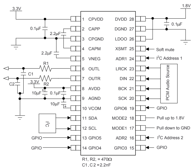
Figure 21. I²C Control, VCOM Mode, DVDD=1.8V
