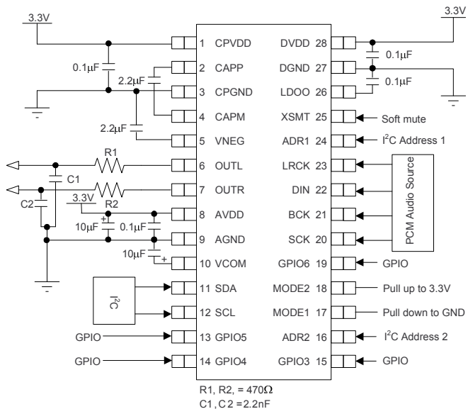
Figure 19. I 2 C Control, VCOM Mode, DVDD=3.3V
