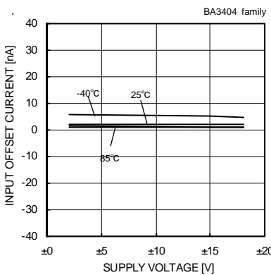
Fig. 107 Input Offset Current - Supply Voltage (Vicm=0[V], VOUT=0[V])
