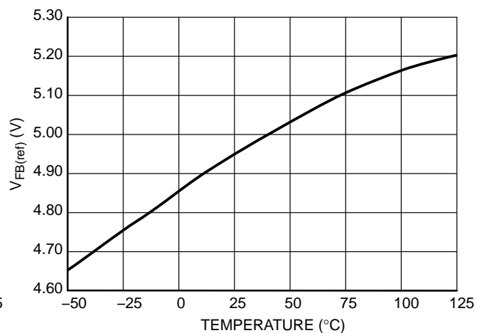
Figure 12. FB Pin Open Voltage V_{\text{FB(ref)}}
