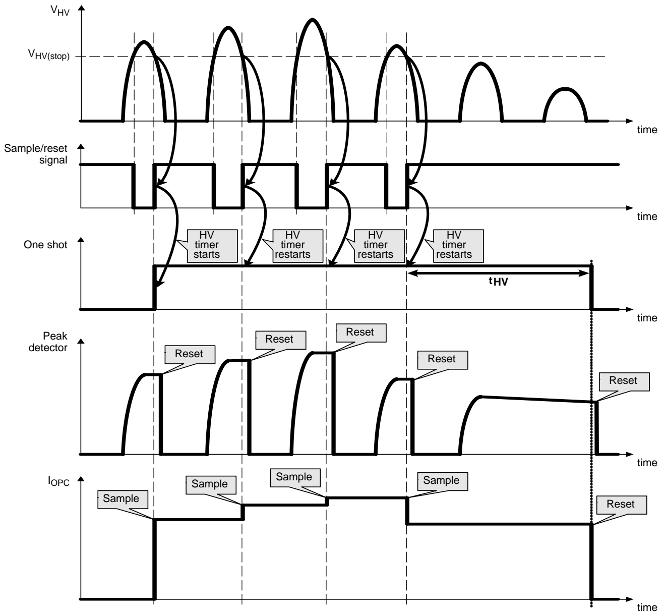
Figure 41. Overpower Compensation
