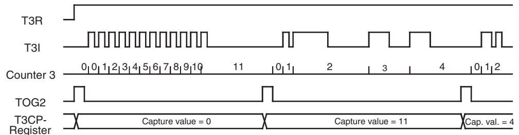
Figure 24-14. Event Counter with Time Gate
