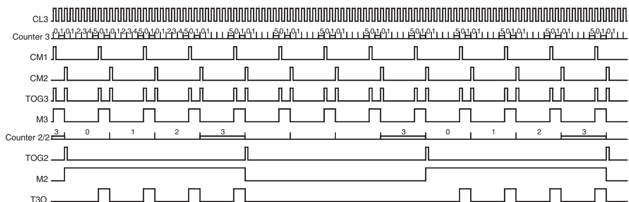
Figure 24-15. Burst Modulation 1
