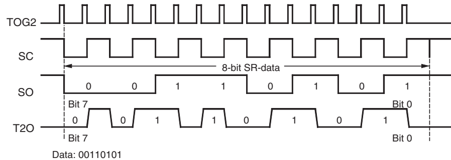
Figure 24-4. Manchester Modulation 1
