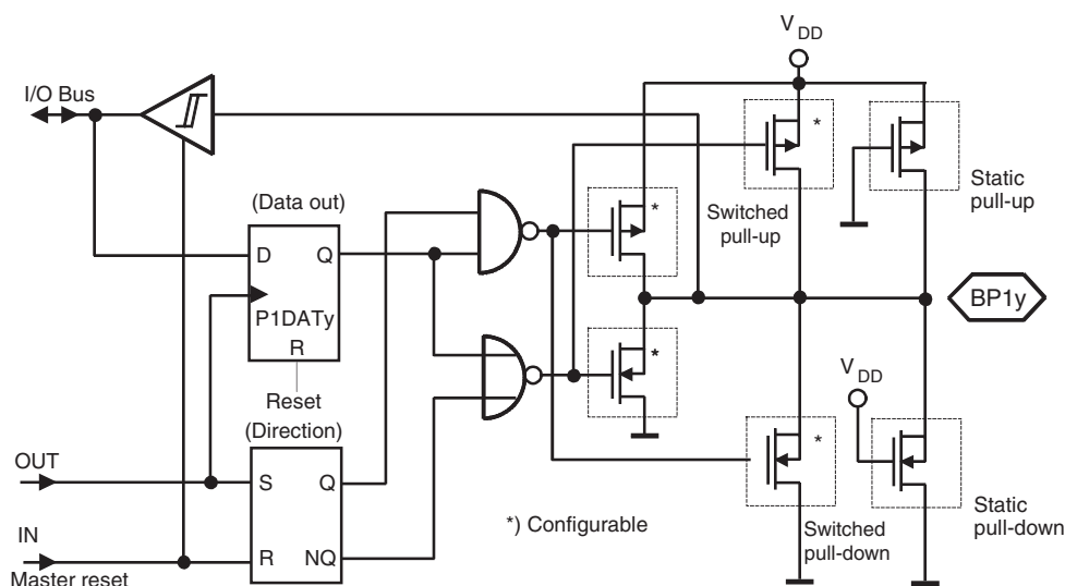
Figure 22-1. Bi-directional Port 1
