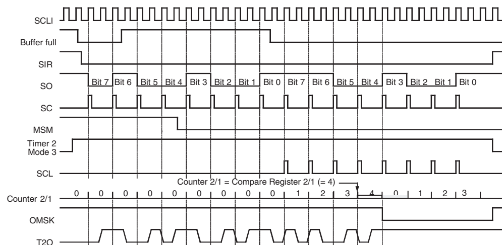
Figure 24-5. Manchester Modulation 2
