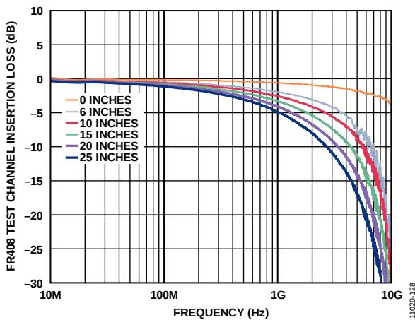
Figure 14. S21 Test Traces
