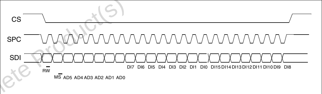
Figure 8. Multiple bytes SPI Write Protocol (2 bytes example)
